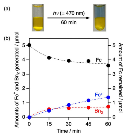
Fig. 2 (a) Photographs of a biphasic solution before and after irradiation, and (b) time course of \text{Fc}^+ /Bn 2 formation and Fc consumption along with Fc conversion from a biphasic H 2 O/DCE solution (1:1, v/v; 2.0 mL) containing Fc (5.0 mM, 5 μmol), Ir (0.05 mM, 50 nmol), and Bn–Br (50 mM, 50 μmol) under visible-light irradiation ( \lambda = 470 \text{ nm} ).
