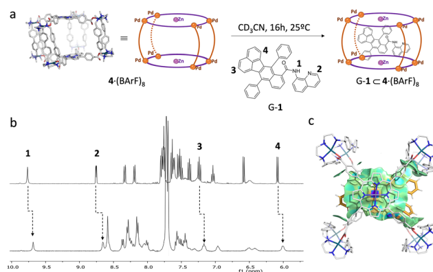
Fig. 1 (a) Schematic representation of the binding of G-1 within cage 4\cdot(\text{BArF})_8 . (b) Stacked partial ^1\text{H} NMR spectra of G-1 (top) and G-1· 4\cdot(\text{BArF})_8 (bottom), showing spectral changes upon host-guest complexation. (c) Representation of non-covalent interaction (NCI) surface of encapsulated G-1 within the cage (weak van der Waals interactions in green and stronger interactions in blue).
