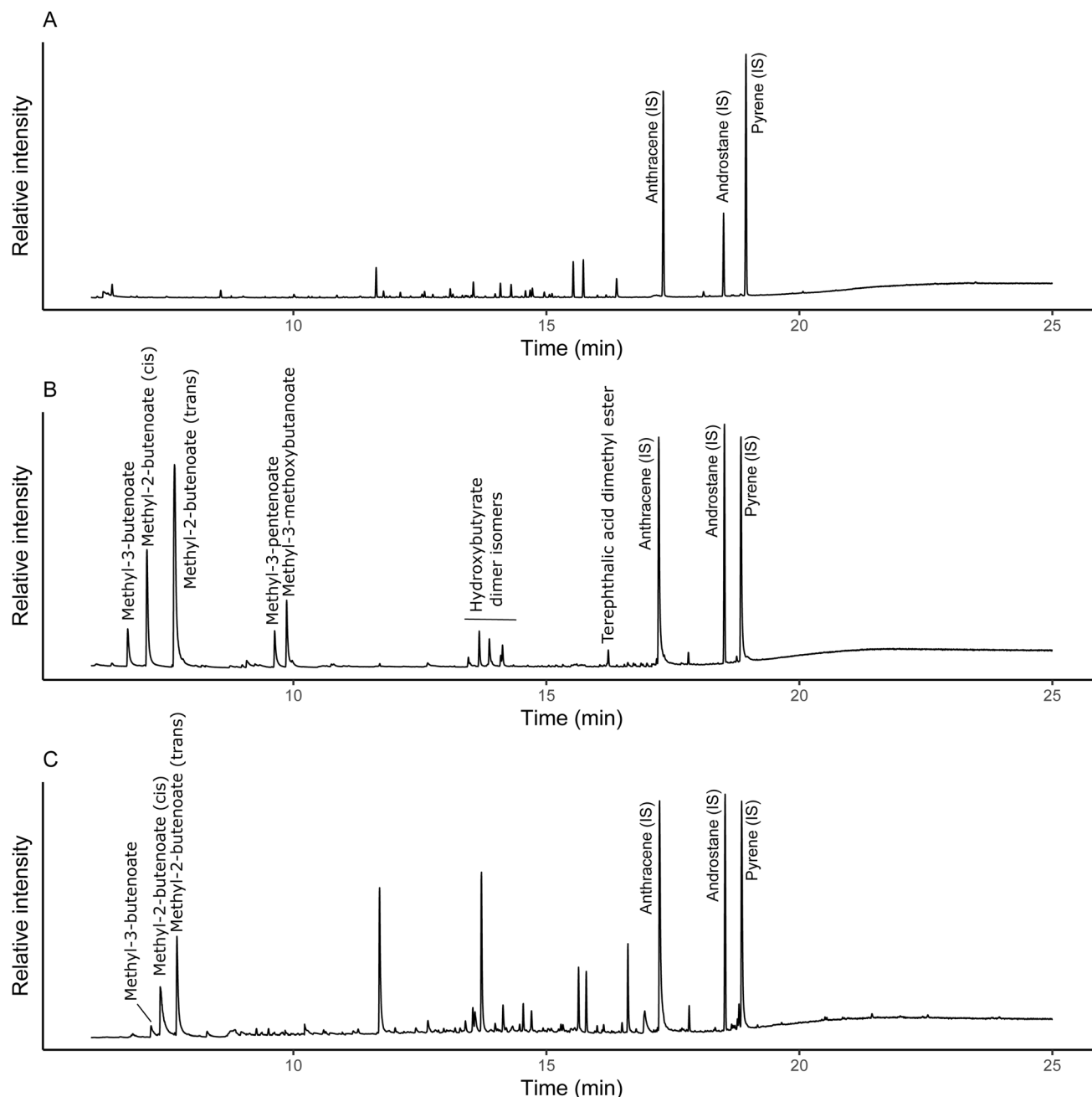
Fig. 1 Partial total ion pyrograms of control soil (A), pure PHBV (41 µg) (B) and soil spiked with 0.1% PHBV (C) pyrolyzed at 350 °C. IS indicates internal standards used to normalise for differences between pyrolysis runs. Unlabelled peaks in (A) and (C) are soil derived compounds.
