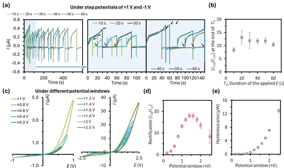
Fig. 4 (a) I - t plots of the bipolar electrochemical memristor under chronoamperometry step potentials of \pm 1\text{ V} with step durations ( T_E ) of 10 s to 60 s and the magnified plots. Black arrows indicate the data taken for calculating |I_{+1V}/I_{-1V}| . (b) Plot of |I_{+1V}/I_{-1V}| against T_E (0.5 mM \text{Na}_2\text{SO}_4 , 10-nm PCTE). (c) I - V plots under potential windows of \pm 0.2\text{ V} to \pm 1\text{ V} and \pm 1.2\text{ V} to \pm 2.5\text{ V} and (d) the corresponding |I_{+1V}/I_{-1V}| and (e) area of the hysteresis loop against the potential window (0.5 mM \text{Na}_2\text{SO}_4 , 0.04\text{ V s}^{-1} , 10-nm PCTE).
