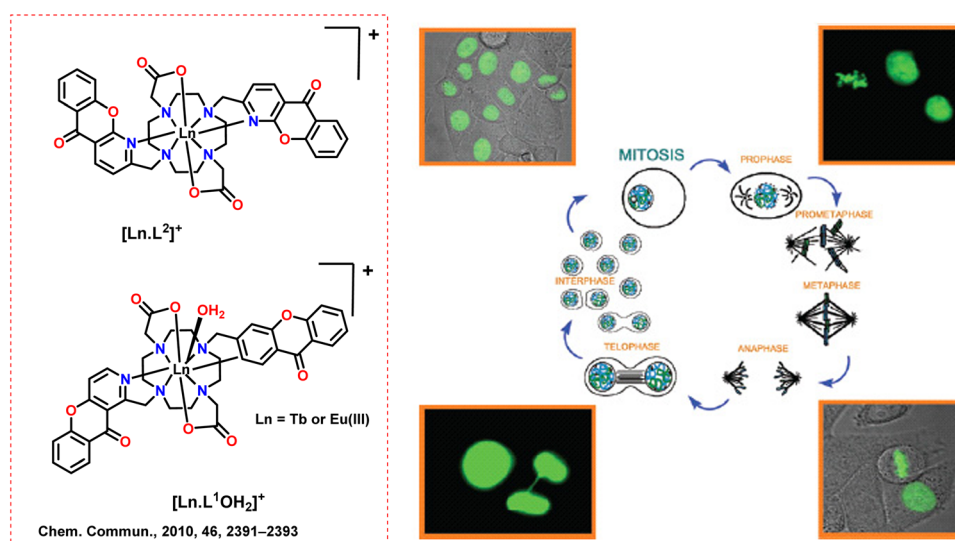
Scheme 14 (Left) Molecular structures of some cyclen-based ligands and chiral Ln complexes ([Ln(L) 2+ ] + and [Ln(L 1 OH 2 ) + ] + ). 71 (Right) Bright field (upper left and lower right) and fluorescence microscopy images of HeLa cells undergoing mitosis, with an illustrative of the cell cycle (0.5 mM, [Tb(L) 2+ ]Cl, 3 h, \lambda_{\text{exc}} 350 nm). Reproduced from ref. 71 with permission from the Royal Society of Chemistry, copyright [2010]. 71
