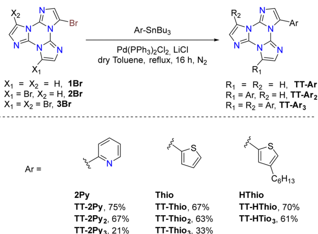
Scheme 5 Synthesis of TT derivatives by Stille cross-coupling.
