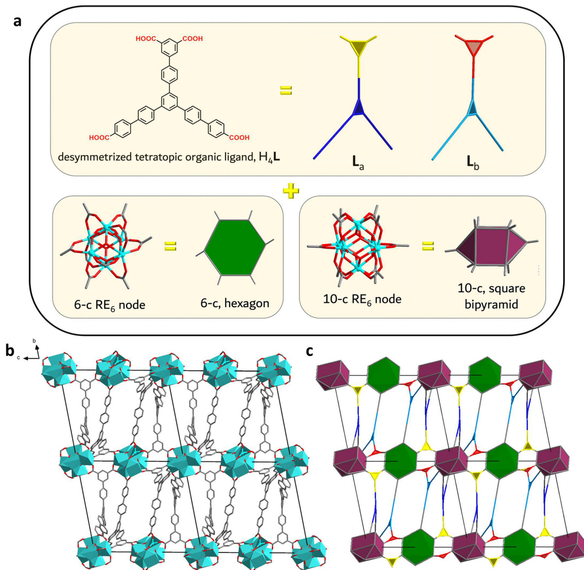
Fig. 2 (a) The combination of the desymmetrized, tetratopic H_4L organic linker with 6-c and 10-c RE_6 -clusters resulted in the formation of RE- stc -MOF-1 series of MOFs. Their geometric representation used for the topological analysis is shown where crystallographically distinct components have different colors. (b) The structure of Eu- stc -MOF-1 looking down the a -axis. (c) The unique six nodal, (3,3,3,3,6,10)-c, augmented stc -a net derived from the topological analysis of Eu- stc -MOF-1.
