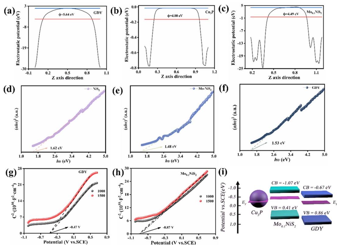
Fig. 10 Work functions of (a) GDY, (b) \text{Cu}_3\text{P} and (c) \text{Mo}_{0.1}\text{NiS}_2 ; bandgap structure diagram of (d) \text{NiS}_2 , (e) \text{Mo}_{0.1}\text{NiS}_2 and (f) GDY; Mott–Schottky plots of (g) GDY and (h) \text{Mo}_{0.1}\text{NiS}_2 at different frequencies; and (i) band structure diagram between CGM-10.
