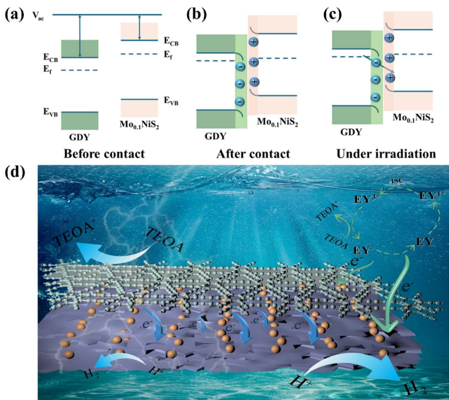
Fig. 11 (a–c) Schematic diagram of charge transfer mechanism between CGM-10; and (d) diagram of the mechanism of \text{H}_2 evolution in sunlight.
