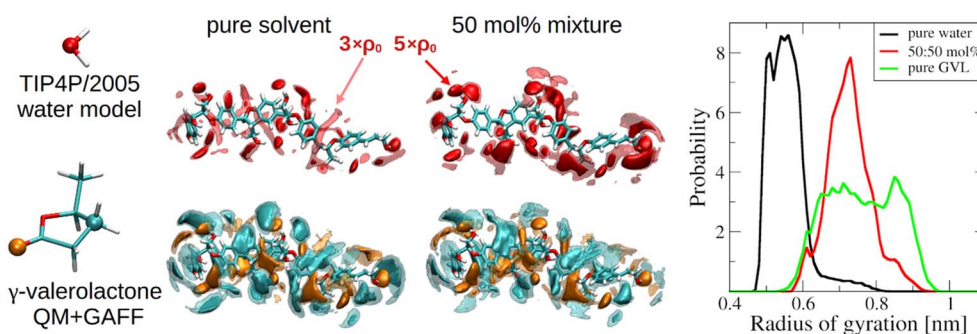
Fig. 3 Synergy in hydration and solvation of a swollen configuration ( R_g \sim 0.85 nm) of PCA-5mer in pure solvents (left) and in their 50 mol% ( ca. 85 w%) mixture (right). Spatial distribution of water (oxygen in red), polar carbonyl oxygen of GVL (in gold), and non-polar carbon atom of GVL (in cyan) are shown at two isocontour levels; 3× and 5× increased probabilities are denoted as transparent and opaque clouds (as illustrated by red arrows on water oxygen distributions). Compared to pure solvents, both water hydration of hydroxyl groups and hydrophobic interaction of GVL with hydrophobic moieties are significantly strengthened, with mild decrease of GVL carbonyl H-bonding interaction with hydroxyl groups. Impact of solvent quality (water vs. GVL) on a PCA-5mer conformation is captured in distribution of polymer size (radius of gyration), in the most right panel. Visualization of the regions of increased density of solvent molecules, analysis for collapsed configuration of PCA-5mer and comparison of solvation of rigid structures to flexible ensembles are provided in detail in the SI Section S6.
