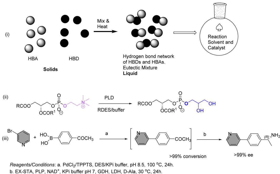
Fig. 1 (i) Formation of NADESs from HBA and HBD building blocks. (ii) The use of RDES in biocatalytic phospholipid preparation. (iii) A sequential metal-catalyzed/biocatalyzed transamination.
