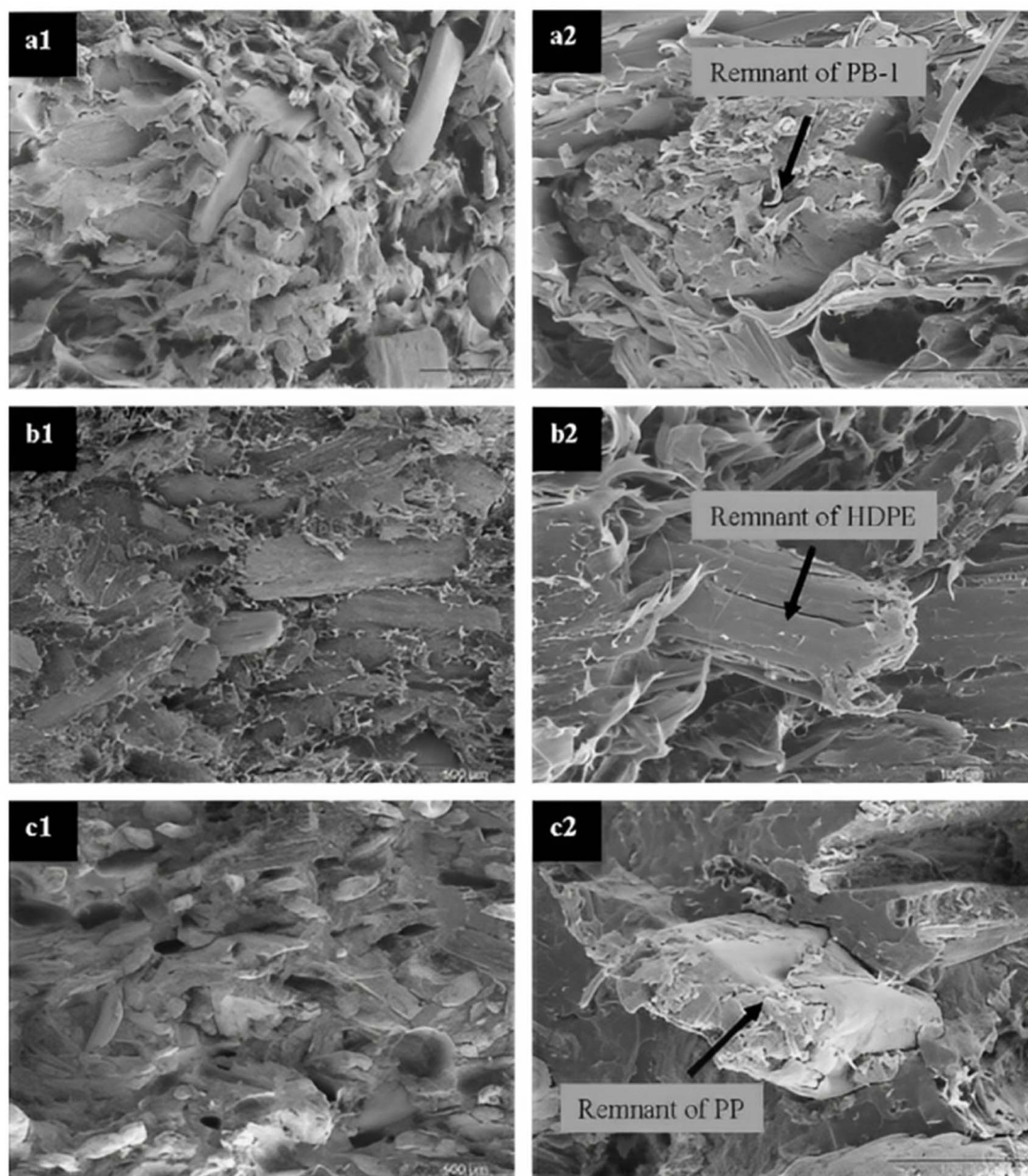
Fig. 13 SEM images of WPCs at two magnifications (50× and 400×) (a1 and a2) PB-I, (b1 and b2) HDPE, and (c1 and c2) PP. Reprinted with permission. 107 Copyright 2010, Elsevier.
