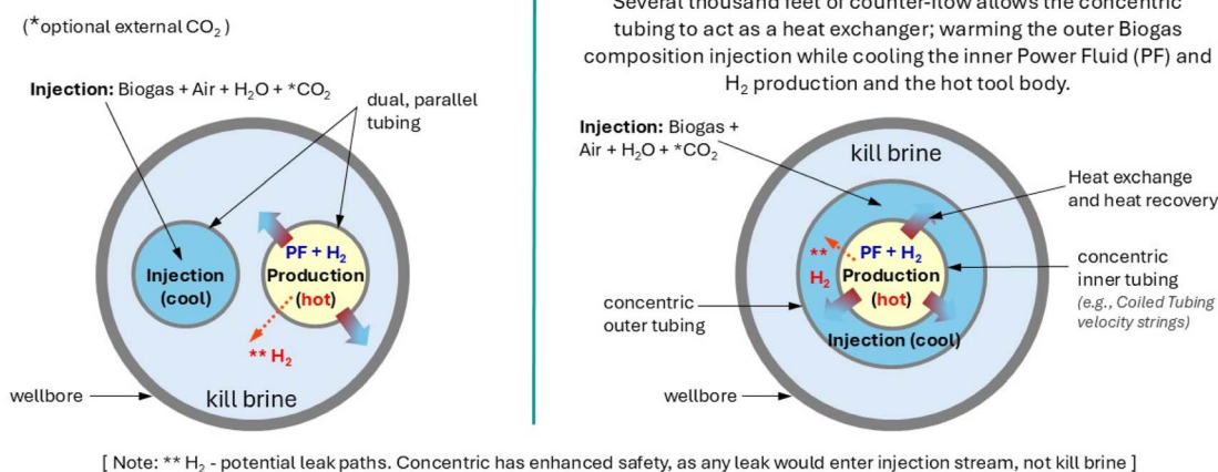
Fig. 6 Dual versus concentric tubing, highlighting safety and heat transfer benefits.
