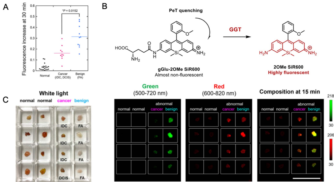
Fig. 31 Application of fluorescent probes for optical discrimination of breast cancer and benign breast lesions. (A) Fluorescence increase of HMR \alpha Man in normal, malignant (IDC, DCIS), and benign (FA) tissues. The probe showed stronger signals in FA than in cancer tissues. (B) A newly developed activatable red fluorescent probe for GGT, gGlu-2OMe SiR600, with fluorescence quenched via PeT. (C) White light (left) and dual-color fluorescence images (right) of normal, malignant, and benign tissues acquired 15 min after administration of both probes. Adapted with permission from ref. 158 Copyright 2020, American Chemical Society.
