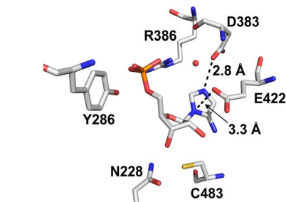
Fig. 7 Crystal structure of the AtThiC active site with AIR bound. Distances of E422 and D383 to the aminoimidazole group are labeled. PDB 4S27. 16
