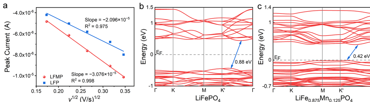
Fig. 2 (a) Plots of the current of the reduction peak ( I_p ) of LFMP and LFP versus the square root of the electrode scanning rate ( v^{1/2} ). Energy band diagrams of LFP (b) and LiFe_{0.875}Mn_{0.125}PO_4 (c).
