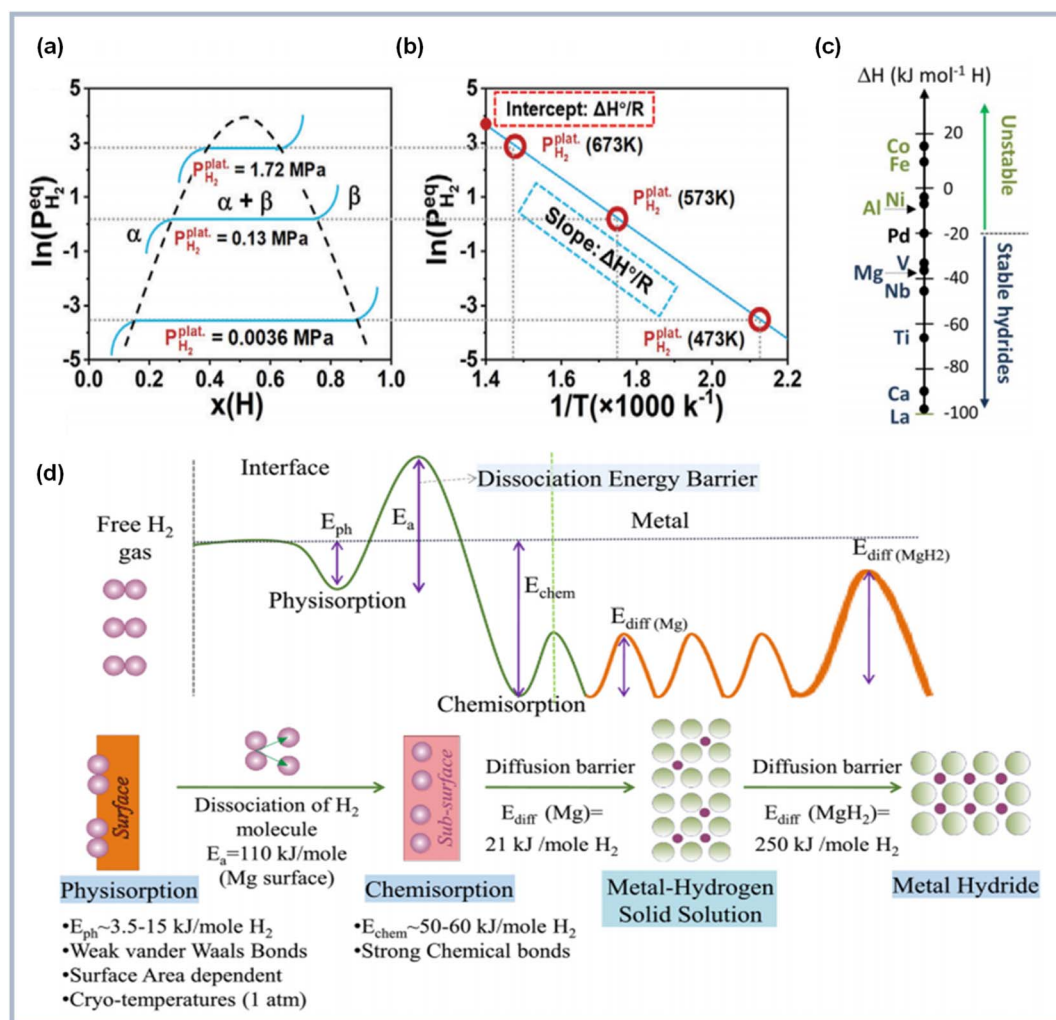
Fig. 3 (a) Pressure–composition isotherm plot of Mg + H 2 ⇌ MgH 2 transition (b) van't Hoff plot related to the phase transition of Mg + H 2 ⇌ MgH 2 ; 49 (c) enthalpy of formation of various metal hydrides; 50 (d) schematic diagram describing continuous energy barriers in the process of hydrogen absorption (up) and illustration of the kinetic steps in the hydrogen storage process (down). 51
