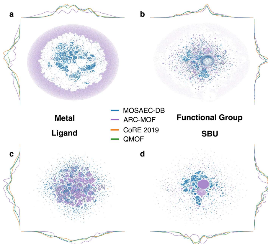
Fig. 6 Comparison of the two-dimensional projections of revised autocorrelation (RAC) descriptor space computed within the MOSAEC, ARC-MOF, CoRE 2019, and QMOF databases. Probability density distributions across each of the reduced t-SNE axes are depicted to provide additional contrast between the datasets. The (a) metal, (b) function group, (c) ligand, and (d) SBU RAC descriptors subcategories are distinctly characterized to display the relative coverage of each database in various domains of chemical space. Dimensionality reduction is performed using the t-SNE algorithm on the combined descriptor space of all relevant structures.
