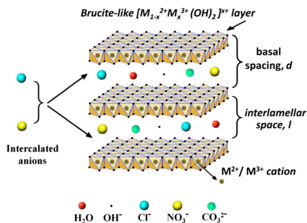
Fig. 2 Schematic structure of M^{2+}/M^{3+} layered double hydroxides (LDHs), showing the brucite-like layers with charge-balancing anions ( \text{Cl}^- , \text{NO}_3^- , \text{CO}_3^{2-} ) intercalated in the interlamellar space, together with water molecules and hydroxyl groups. This layered architecture provides high anion-exchange capacity and tunable interlayer spacing, enabling LDHs to act as versatile carriers for negatively charged nutraceuticals, antioxidants, and preservatives. The intercalation ability illustrated here underpins their role in controlled release and stabilization within food and packaging applications. The figure is obtained from ref. 34 under a Creative Common (CC BY) License.
