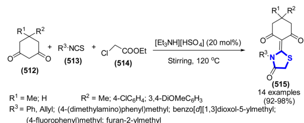
Scheme 136 Synthesis of thiazolidine/oxazolidine derivatives catalyzed by [Et_3NH][HSO_4] .
