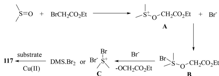
Scheme 47 Copper-assisted C5 bromination of 8-aminquinoline amide using alkyl bromide.
