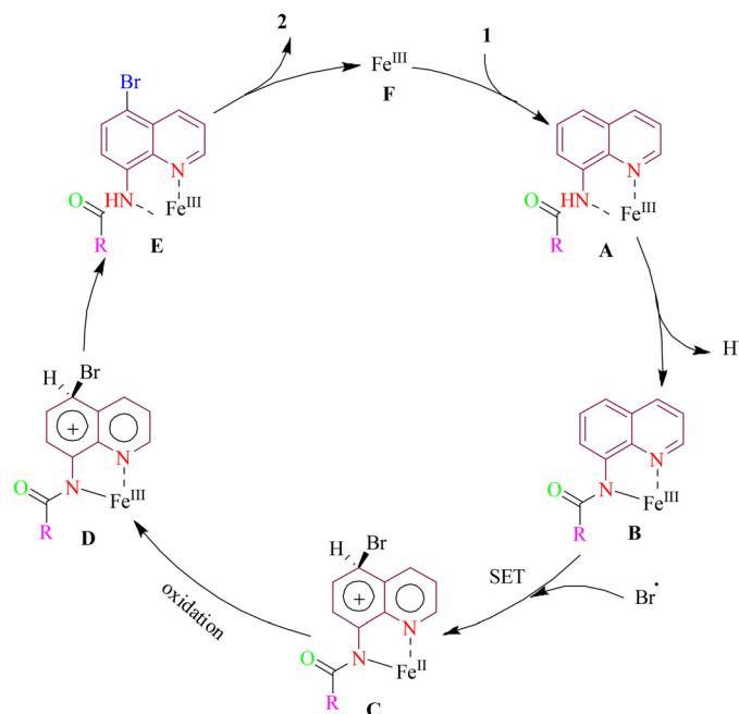
Scheme 1 Fe(III)-catalyzed C-5 halogenation of 8-aminoquinoline amide.
