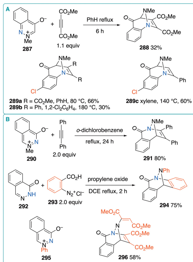
Fig. 40 (A) (5 + 2) cycloaddition of 2-methyl-4-oxidocinnolinium betaines with alkynes. (B) (5 + 2) cycloaddition of 1-oxidophthalazine betaines with alkynes and benzyne.
