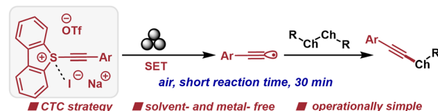
Fig. 1 (A) Piezoelectric material-catalyzed radical reactions via ball milling, (B) generation of the super electron donor phenalenyl anion via ball milling, and (C) this work: charge transfer complex enabled radical alkynylations via ball milling.
