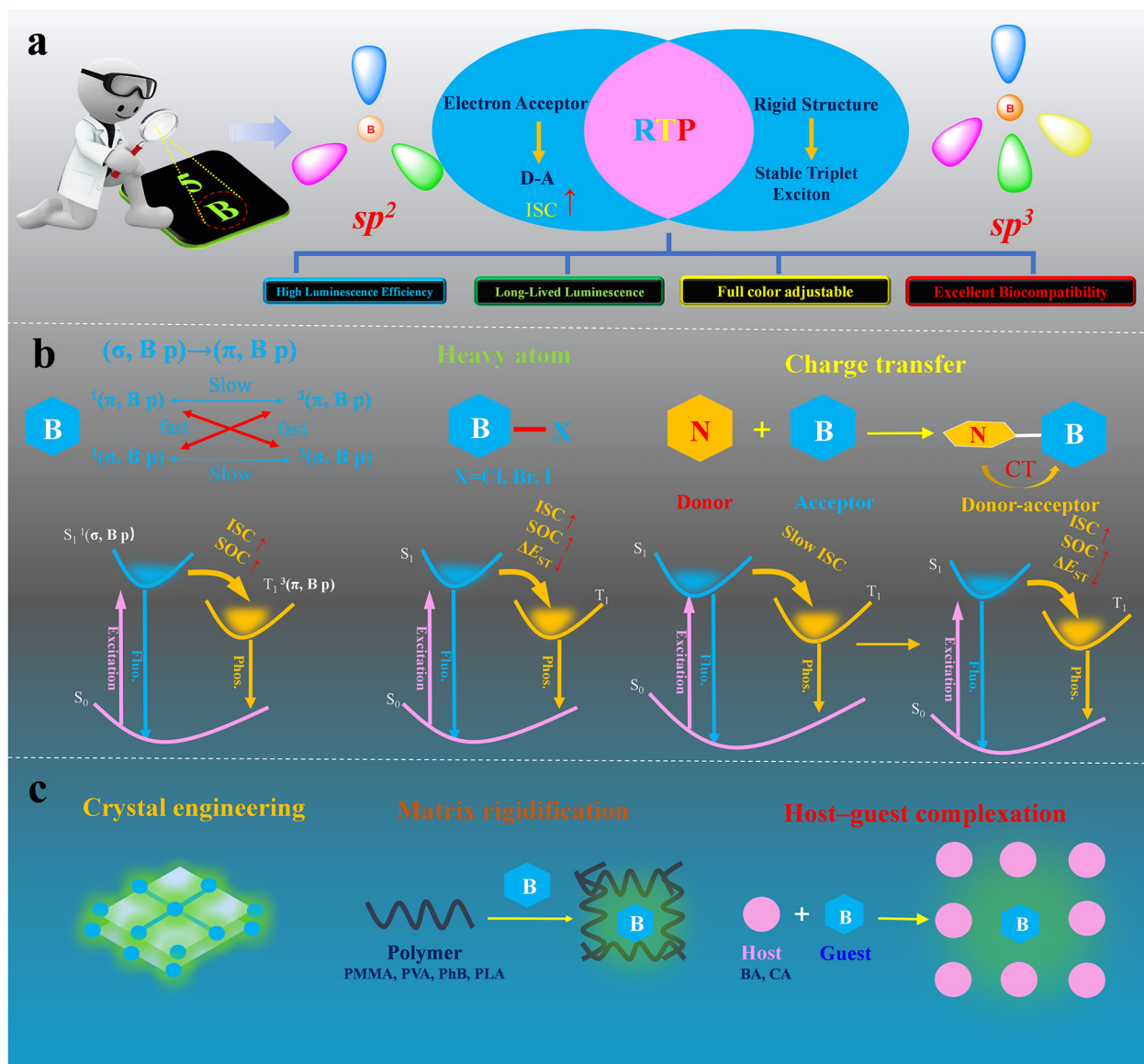
Fig. 1 (a) Boron-based room temperature phosphorescent materials; (b) strategies of molecular design, including the ( \sigma, B p ) \rightarrow ( \pi, B p ) transition mechanism in three-coordinate boron systems, heavy atom introduction, and donor-acceptor system design to facilitate ISC and stabilize triplet states; (c) strategies for room-temperature phosphorescence efficiency enhancement, such as crystal engineering, host-guest doping, and suppression of non-radiative decay via rigidification.
