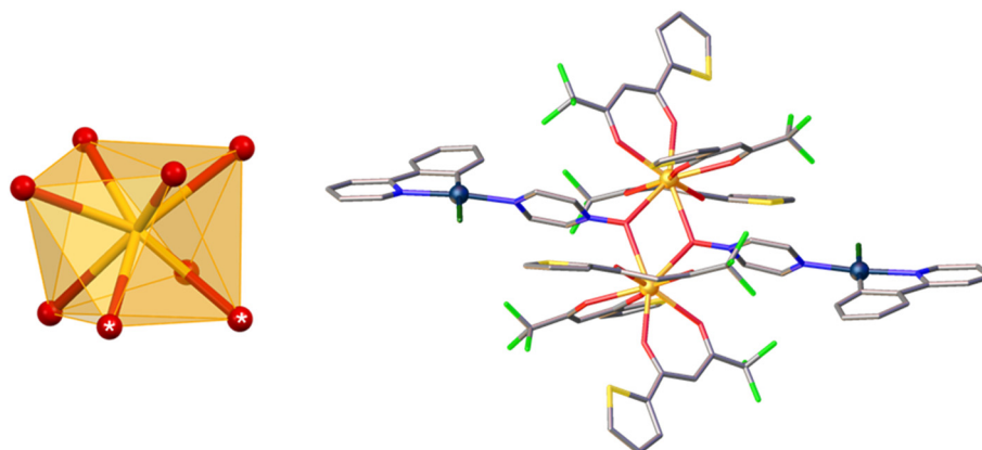
Fig. 3 Molecular Structure and coordination polyhedron of the \text{EuO}_8 core for 6 . Hydrogen atoms and disordered parts are omitted for clarity. Colour code: C, grey; O, red; N, blue; S, yellow; F, light green; Cl, dark green; Pt, dark blue; Eu, orange. Oxygen atoms marked with the white asterisk belong to the bridging pyrzMO units.
