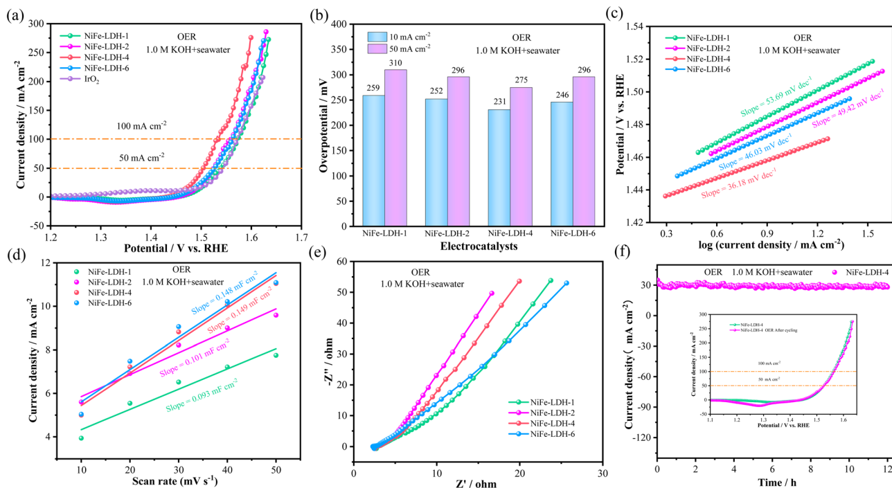
Fig. 5 OER performance in seawater (a) polarization curves at scan rate of 5 \text{ mV s}^{-1} (b) bar chart (c) Tafel plots (d) CV curves of double-layer capacitance ( C_{\text{dl}} ) (e) Nyquist plots (f) chronoamperometric stability tests the insets is LSV curves before and after cycle.
