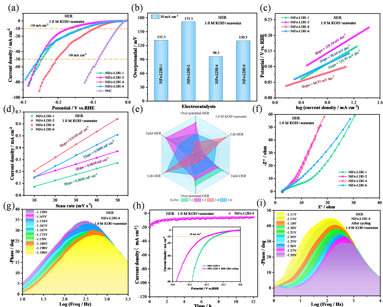
Fig. 6 HER performance in seawater (a) polarization curve at a scanning rate of 5 mV s -1 (b) bar chart (c) Tafel plot (d) CV curve of double-layer capacitor (C dl ) (e) HER and OER radar plot (f) Nyquist plot (g) Bode plot of NiFe-LDH-4 sample before cycling at multiple voltages (h) timing current stability test illustration LSV curve before and after cycling (i) Bode plot of NiFe-LDH-4 sample after cycling at multiple voltages.
