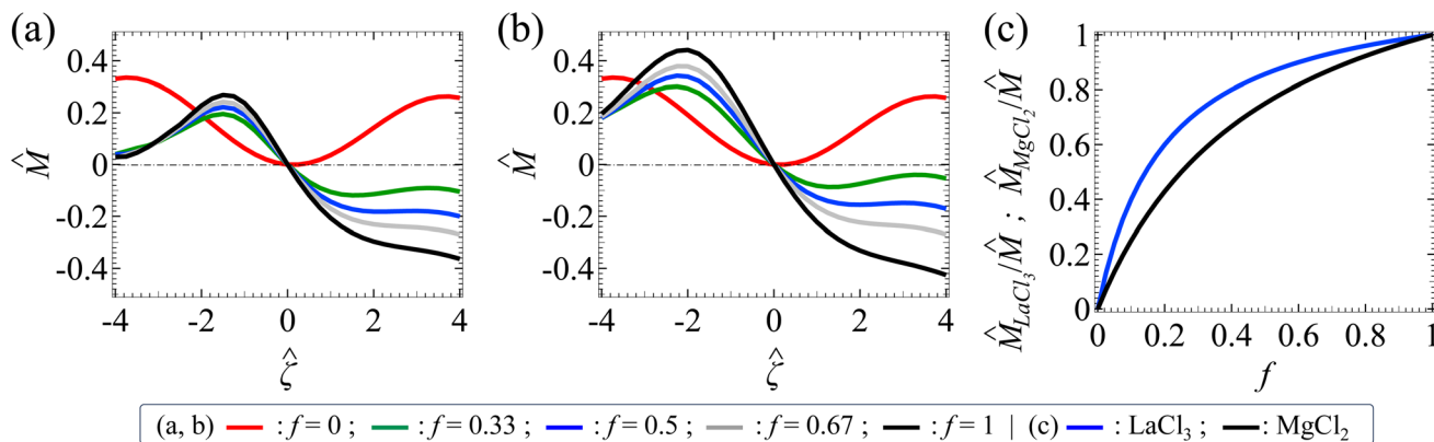
Fig. 5 (a) The non-dimensionalized diffusiohoretic mobility \hat{M} versus the non-dimensionalized colloid surface potential \hat{\zeta} in the same porous media (the ratio of the screening length to the colloid radius l/a = 0.75 ) saturated with solution mixtures of p molar of KCl and q molar of LaCl 3 with different compositions f = q/(p + q) . The solution ionic strength I = 1 mM. Red line: f = 0 . Green line: f = 0.33 . Blue line: f = 0.5 . Grey line: f = 0.67 . Black line: f = 1 . (b) \hat{M} versus \hat{\zeta} in the same porous media ( l/a = 0.75 ) saturated with solution mixtures of p molar of KCl and q molar of MgCl 2 with different compositions f = q/(p + q) . The color scheme and the ionic strength are the same as (a). (c) The ratio of the contribution to the mobility by the asymmetric electrolyte to that by the mixture \hat{M}_{\text{LaCl}_3}/\hat{M} and \hat{M}_{\text{MgCl}_2}/\hat{M} versus f . Blue line: \hat{M}_{\text{LaCl}_3}/\hat{M} . Black line: \hat{M}_{\text{MgCl}_2}/\hat{M} .
