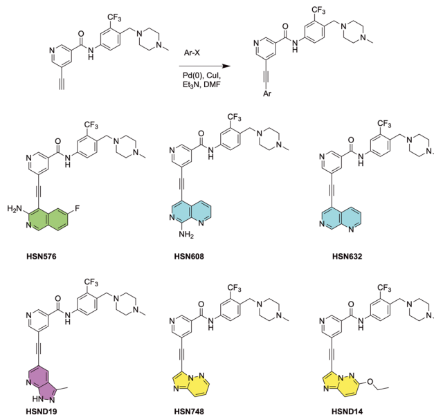
Fig. 1 General synthetic scheme for the synthesis of compounds via Sonogashira reaction and chemical structures of compounds under the study (HSN576, HSN608, HSN632, HSND19, HSN748, HSND14).
