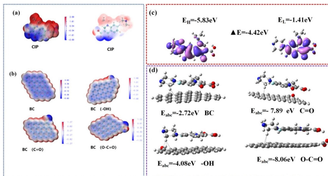
Fig. 11 (a) ESP distribution of CIP, (b) ESP distributions of BC and its functionalized forms (−OH, C=O, and O−C=O), (c) HOMO and LUMO frontier molecular orbitals, and (d) optimized sorption energies and configurations of CIP on biochar with varying oxygen-containing groups (reproduced from ref. 240 with permission from Elsevier, copyright 2025).
