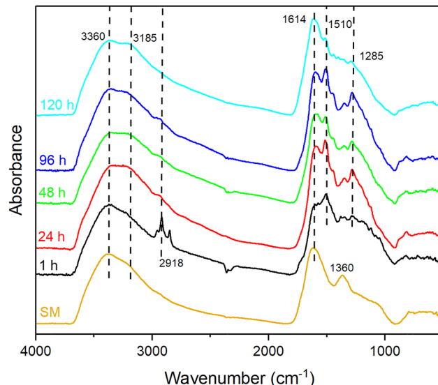
Fig. 8 FTIR absorption spectra of PDA NPs at 1.79% of \text{NH}_4\text{OH} percentage at different reaction time. For comparison, the absorbance spectrum of SM is also shown on the bottom.
