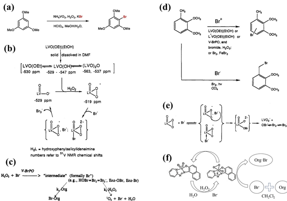
Fig. 1 (a) Reaction equation of \text{NH}_4\text{VO}_3 . 29 Reproduced from ref. 29 with permission from Elsevier, copyright 2022. (b)–(e) Four possible reaction mechanisms of LVO(OEt)(EtOH). 30 Reproduced from ref. 30 with permission from ACS, copyright 1993. (f) Reaction diagram of a tridentate oxygen–nitrogen–nitrogen donor ligand, 1-(2-pyridylazo)-2-naphthol. 32 Reproduced from ref. 32 with permission from Elsevier, copyright 2014.
