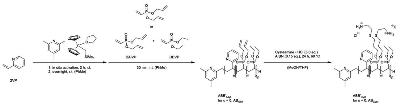
Scheme 1 Synthesis of block copolymers P2VP- b -PDAIVP (AB type, no DEVP added, o = 0 ) and P2VP- b -P(DAIVP- st -DEVP) (ABB' type) using an in situ generated catalyst with subsequent cysteamine modification of the allyl groups of PDAIVP under thiol-ene reaction conditions.
