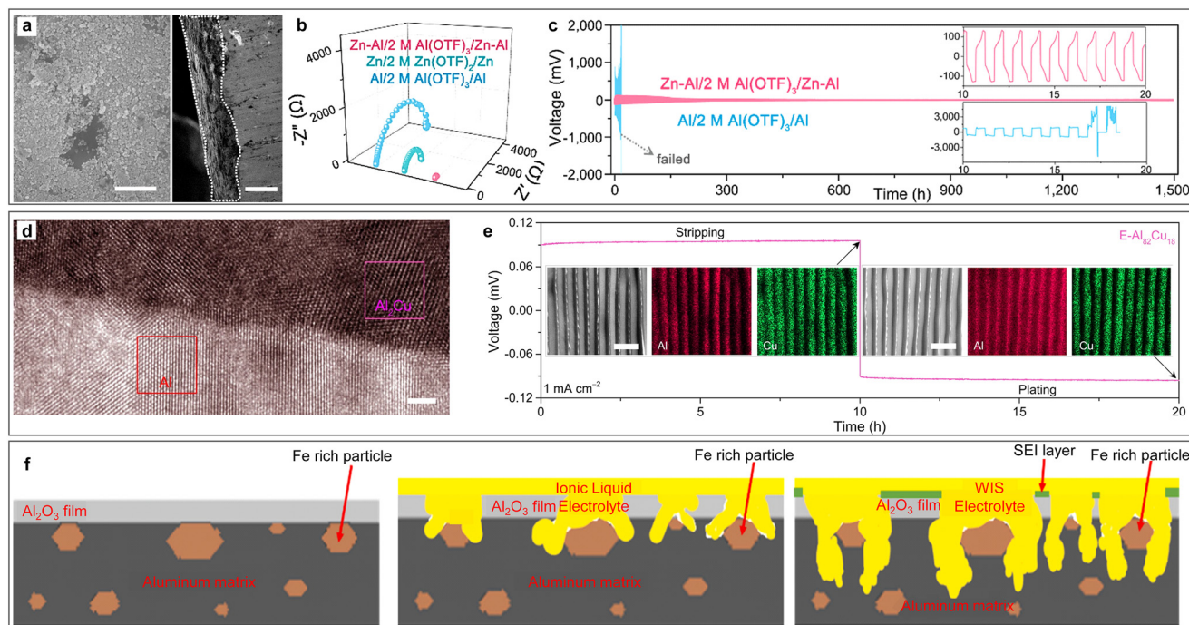
Fig. 6 Aluminium alloy for ARAMBs. (a–c) Zn–Al alloy. (a) SEM images of the top view and cross section of Zn–Al alloy. Scale bars: 500 nm (left) and 30 \mu m (right). (b) Comparative Nyquist plots of symmetrical cells with different electrodes. (c) Comparison of long-term cycling stability for symmetric cells based on Al and Zn–Al alloy electrodes ( 0.2 \text{ mA cm}^{-2} ). Reproduced with permission. 64 Copyright 2020, AMER CHEMICAL SOC. (d and e) Eutectic Al 82 Cu 18 alloy. (d) HRTEM image of Al/Al 2 Cu interfacial region. Scale bars: 2 nm. (e) Stripping/plating voltage profile of E-Al 82 Cu 18 symmetric cells at a current density of 1 \text{ mA cm}^{-2} in 2 M Al(OTF) 3 aqueous electrolytes. Insets: SEM images and corresponding EDS mappings of Al and Cu after stripping (left) and plating (right). Scale bars: 1 \mu m. Reproduced with permission. 66 Copyright 2022, NATURE PORTFOLIO. (f) Schematic illustration of aluminium matrix corrosion during the cycling process in the presence of Al 3 Fe intermetallic phase. Reproduced with permission. 67 Copyright 2022, ELSEVIER.
