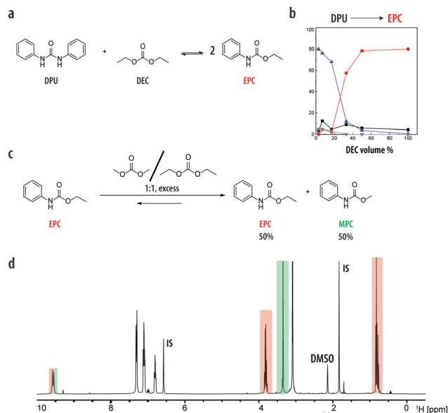
Fig. 3 Carbonyl exchange equilibrium of model compounds N,N -diphenylurea (DPU) and ethyl phenyl carbamate (EPC) with DEC and Zn ( \text{OAc})_2 (■ DPU, ● EPC, ▲ Aniline, ▼ Biuret). (a) Schematic of the equilibrium between a urea (DPU), a carbonate (DEC) and a carbamate (EPC). (b) Relative amounts of DPU and products for reactions performed at varying DEC volume fractions for 4 h (in mixtures with sulfolane). (c) Schematic of the equilibrium between EPC, DEC/DMC and methyl phenyl carbamate (MPC). (d) ^1\text{H} NMR spectrum of the compounds in \text{DMSO}-d_6 after 4 h, EPC : Carbonate ratio 1 : 30, dimethyl carbonate (DMC) : DEC ratio 1 : 1, 10 mg \text{Zn}(\text{OAc})_2 (IS = internal standard).
