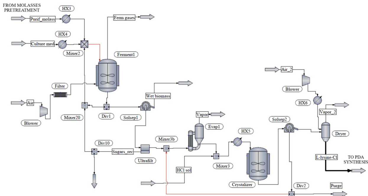
Fig. 3 Flow diagram for the biosynthesis of L-lysine HCl from treated sugarcane molasses.
