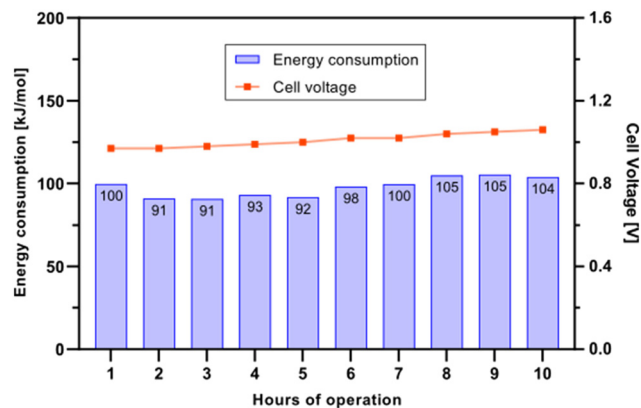
Fig. 8 Cell voltage response and electrochemical energy consumption of a 10 hours measurement with a RSW flow rate of 25 mL \text{min}^{-1} and a current density of 5 mA \text{cm}^{-2} while introducing a 0.5 M HCl wash step every hour for 8 minutes with a flow rate of 45 mL \text{min}^{-1} .
