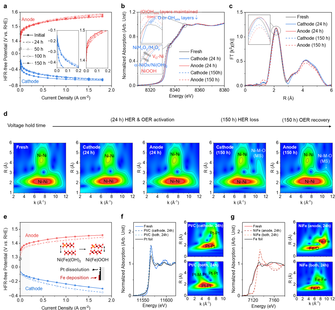
Fig. 4 Study on the activity–structure/property relationship at the cathode and anode under applied cell voltage. (a)–(d) Evolution of potential and properties under a constant 2.0 V voltage hold for up to 150 h without integrated catalysts. HFR-free polarization curves (a). Note that compared to the 100 h measurement, the 150 h results show a slight decrease in HER activity (deactivation) and a slight increase in OER activity (recovery), leading to a modest improvement in the full-cell polarization curve (Fig. S31, SI). Ni K-edge normalized XANES (b), FT-EXAFS (c), and WT-EXAFS (d). Insets in (a)–(c) provide magnified views of each plot. (e)–(g) Potential and property changes before and after a 24 h 2.0 V hold in the Pt/C + NiFe (both) case. HFR-free polarization curves (e). The schematic in (e) illustrates the anticipated changes in the Pt/C cathode catalyst layer and the NiFe anode catalyst layer after voltage application. Pt L-edge normalized XANES ((f), left) and WT-EXAFS ((f), right) for the cathode. Fe K-edge normalized XANES ((g), left) and WT-EXAFS ((g), right) for the anode.
