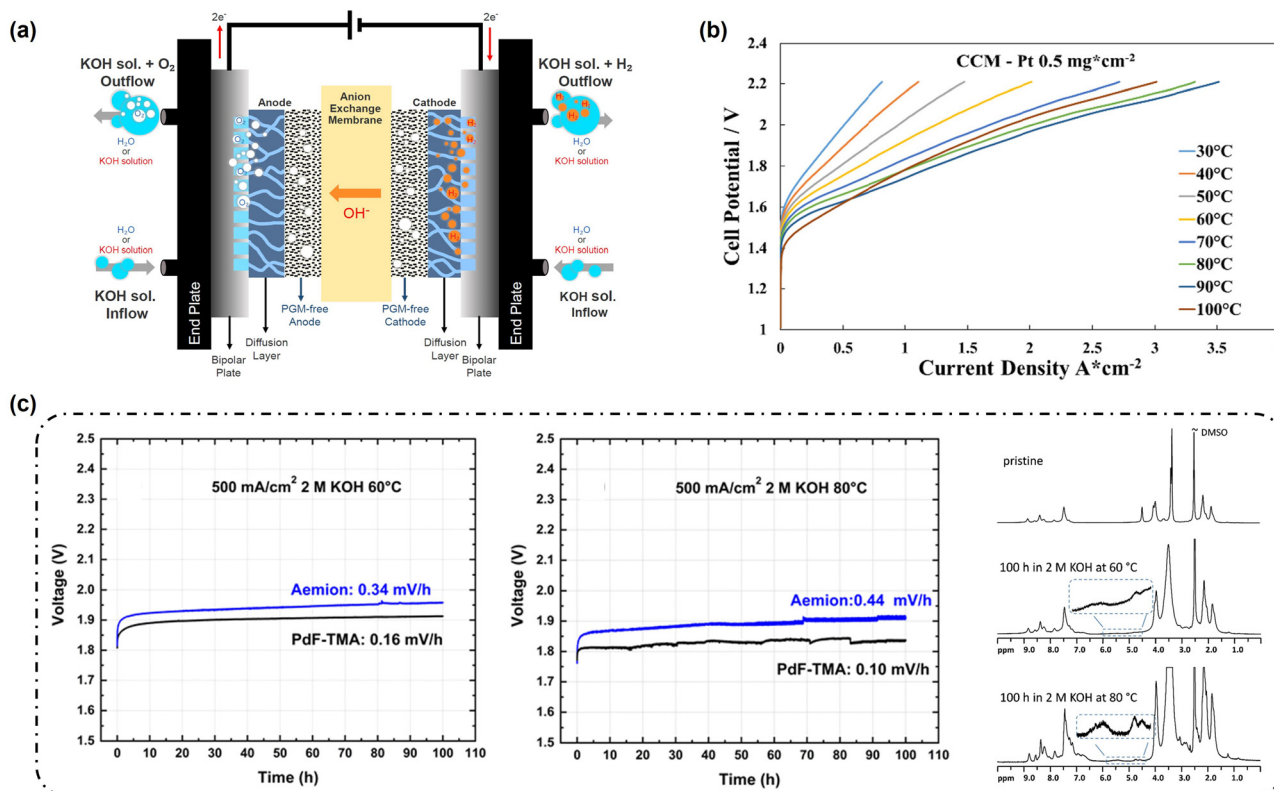
Fig. 23 (a) Schematic diagram of the AEMWE. 257 (b) Polarization curves for AEMWE on the CCM configuration at different temperatures. 258 (c) Stability evaluations at 500 mA cm -2 in 2 M KOH at 60 °C and 80 °C and 1 H NMR spectra of the Aemion membrane before and after long-term stability evaluation in the electrolysis cell. 259
