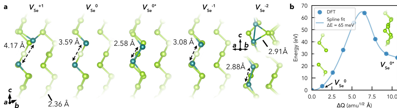
Fig. 5 (a) Geometries of the intrinsic vacancy ( V_{Se} ) in t-Se, under various charge states, looking down the 83 Se lattice direction. The two neighbouring Se atoms to the vacancy site are shown in teal as a guide to the eye. V_{Se}^{0*} refers to the metastable neutral vacancy, and V_{Se}^{-2} is additionally shown along the [110] direction to make the bridging bonds between Se chains visible. (b) Potential energy surface along the lowest energy path between the ground-state ('split'/bipolaron') V_{Se}^0 and metastable ('self-healed') V_{Se}^{0*} structures, calculated using hybrid DFT including spin-orbit coupling within the nudged elastic band (NEB) approach.
