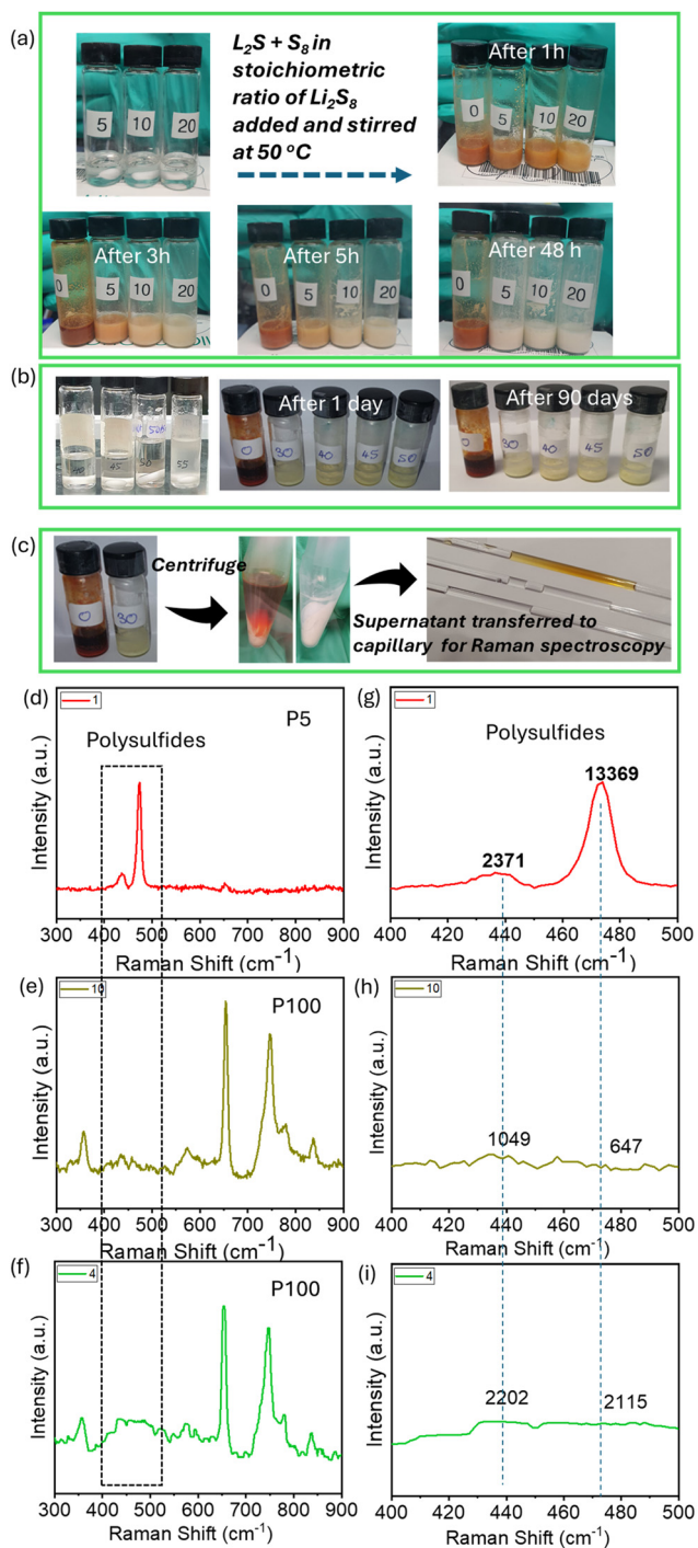
Fig. 2 Polysulfide dissolution test: (a) display of the color change of neat-IL and low-concentration electrolytes (0, 5, 10 and 20 mol% LiTFSI in P 1114 FSI IL) after the addition of Li 2 S and sulfur powder at 50 °C. (b) Display of the color change of neat-IL and moderate and high-concentration electrolytes (0, 30, 40, 45 and 50 mol% LiTFSI in P 1114 FSI IL) before and after the addition of Li 2 S and sulfur powder at 50 °C. (c) Steps of sample preparation for Raman-spectroscopy. Raman spectra of (d) Li 2 S + S in P 1114 FSI IL by utilizing 5% of LAZER power (e) Li 2 S + S in 30 mol% LiTFSI in P 1114 FSI IL by utilizing 100% of LAZER power (f) 30 mol% LiTFSI in P 1114 FSI IL by utilizing 100% of LAZER power. (g, h, and i) are the zoomed view of (d, e, and f) respectively.
