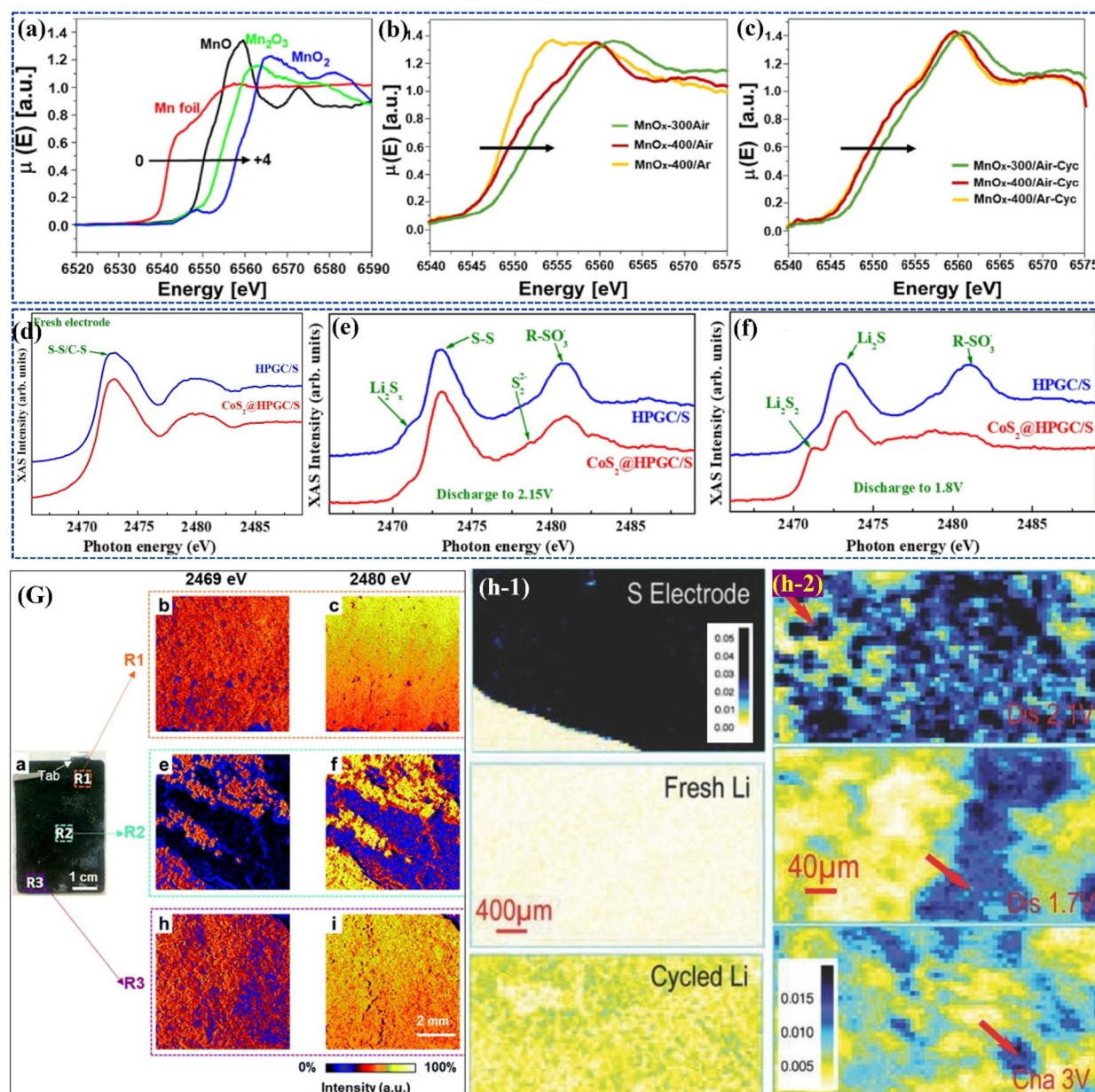
Fig. 9 Mn K-edge XANES spectra for (a) Mn reference compounds, (b) fresh and (c) cycled electrodes. Reproduced with permission. 132 Copyright 2023, Elsevier. TFX-NEXAFS spectra of the S K-edge (d) fresh electrode and cycled electrode discharged to (e) 2.15 V and (f) 1.8 V. Reproduced with permission. 133 Copyright 2019, American Chemical Society. (G) Revealing the local chemical nature of cycled S cathode by combined XRF and XAS analysis. Reproduced with permission. 134 Copyright 2020, Royal Society of Chemistry. (h-1) XRF images collected on sulfur/Ketjen black electrode, fresh Li foil, and cycled Li foil after one cycle. (h-2) XRF images collected on lithium anode electrodes harvested from the Li/Sulfur/Ketjen black cells at discharged 2.1 V, discharged 1.7 V, and re-charged 3 V states. Reproduced with permission. 135 Copyright 2015, Wiley-VCH.
