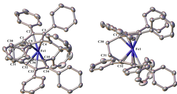
Fig. 5 ORTEP diagram of complex 5·2 THF showing atom-numbering scheme for relevant atoms. Left: showing the \eta^5 coordination mode of Cp to Fe; right: showing the ansa bridge. Thermal ellipsoids are drawn at the 50% probability level. Hydrogen atoms and lattice solvent are omitted for clarity. Selected bond lengths (Å): C(1)–Fe(1) 2.000(2), C(2)–Fe(1) 2.074(2), C(3)–Fe(1) 2.107(2), C(4)–Fe(1) 2.096(2), C(5)–Fe(1) 2.098(2), C(32)–Fe(1) 1.996(2), C(33)–Fe(1) 2.072(2), C(34)–Fe(1) 2.113(2), C(35)–Fe(1) 2.101(2), C(36)–Fe(1) 2.089(2), Fe(1)–Cn(1) 1.676(1), Fe(1)–Cn(2) 1.676(1).
