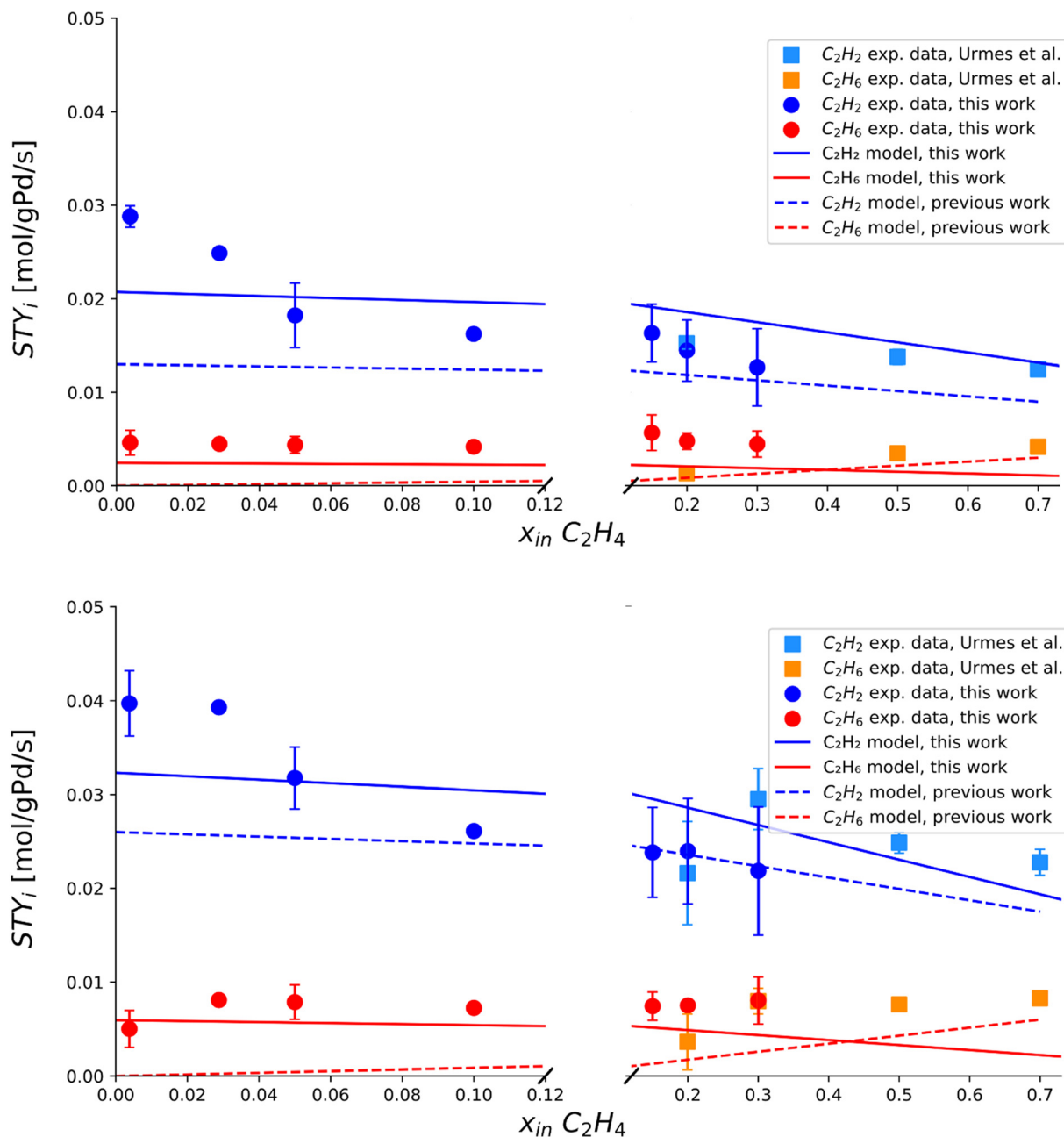
Fig. 7 Experimentally measured and modelled space-time yields of C_2H_2 and C_2H_6 ( STY_{C_2H_2} [ mol\ g_{Pd}^{-1}\ s^{-1} ] and STY_{C_2H_6} [ mol\ g_{Pd}^{-1}\ s^{-1} ]) plotted against the inlet molar fraction of C_2H_4 . Top) Trend obtained at 323 K, i.e. 50 °C. Bottom) Trends obtained at 333 K, i.e. 60 °C. The x-axis is reported with a broken plot representation to precisely quantify the behavior across the composition range investigated. Includes experimental data by Urmès et al., experimental data from this work, model simulation results by this work and a dotted line showing model simulation results by Urmès et al. 11 The standard deviation of experimental measurements is reported through error bars for points whose reproducibility has been verified through at least two repeated experiments.
