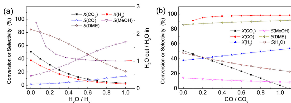
Fig. 5 Effect of a) H 2 O or b) CO addition to feed on equilibrium product distribution in CO 2 hydrogenation to DME. Reaction conditions: 473 K, 3 MPa, H 2 /CO 2 = 4. Copyright 29 2017 Earth and Environmental Science.
