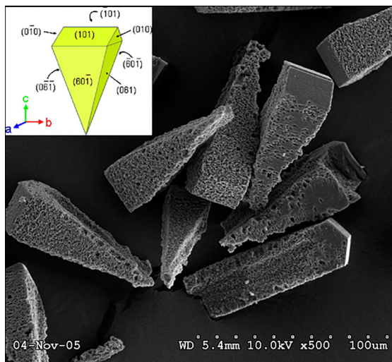
Fig. 24 SEM images of wedge shaped (pyramidal) ZSM-5 crystals, cut perpendicular to the c-axis. The inset shows typical morphology of the pyramidal segment. 557 Reproduced from ref. 557 with permission from the American Chemical Society, copyright 2007.
