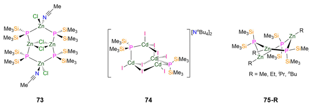
Fig. 21 Group 12 P'' cluster complexes [(Zn(Cl)(MeCN)(μ-P'')) 2 {Zn(μ-Cl)} 2 ] (73), [N''Bu 4 ] 2 [Cd 4 (I) 8 (P'')] (74), [Zn(R)(P'')] (75-R; R = Me, Et, i Pr, n Bu).
