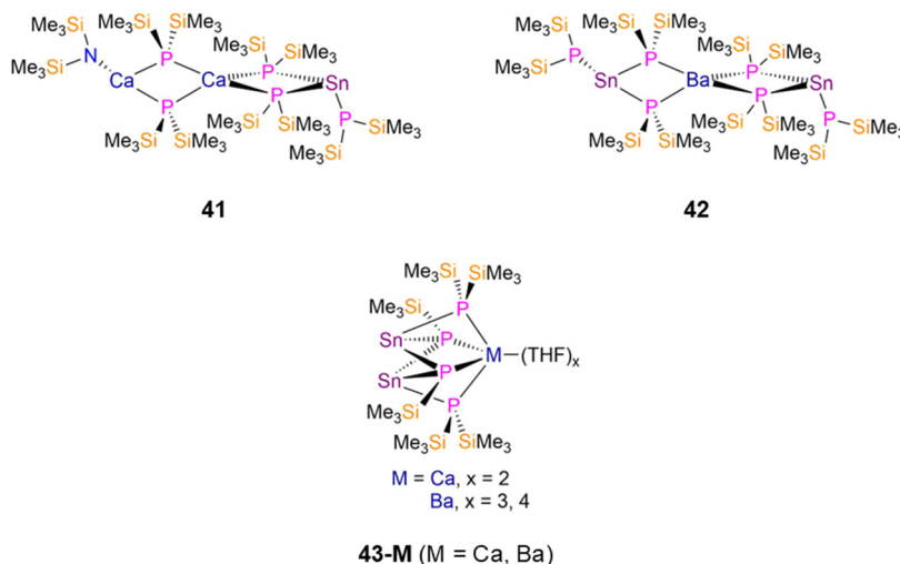
Fig. 12 Heterometallic group 14 P'' complexes [Sn(P'')(μ-P'')_2Ca(μ-P'')_2Ca(N'')] ( 41 ), [Sn(P'')(μ-P'')_2Ba] ( 42 ), [M(THF)_x\{Sn(μ_2-P'')(μ_3-P'')\}_2] ( 43-M ; M = Ca, x = 2 , M = Ba, x = 3, 4 , P'' = \{P(SiMe_3)\} ).
