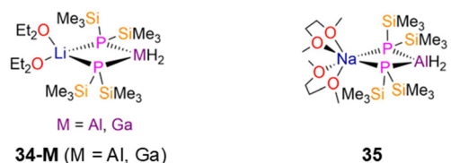
Fig. 9 Heterometallic group 13 \text{P}'' complexes [\text{M}(\text{H})_2(\mu\text{-P}''\text{Li}(\text{Et}_2\text{O})_2)] ( 34-M ; M = \text{Al} , \text{Ga} ), [\text{Al}(\text{H})_2(\mu\text{-P}''\text{Na}(\text{DME})_2)] ( 35 ).
