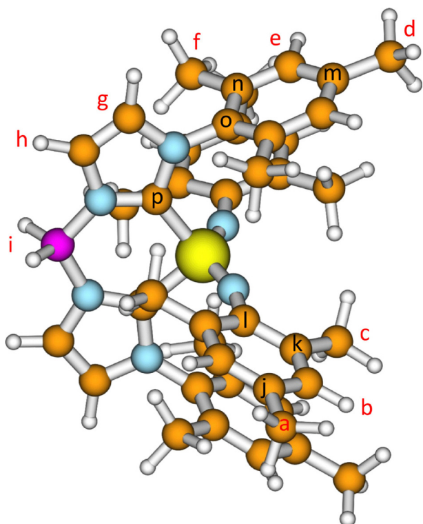
Fig. 1 Schematic illustration of the Fe bisimido complex including labelling of the ^1\text{H} NMR centres in red and the additional ^{13}\text{C} centres in black letters. Iron atom in yellow, boron in purple, nitrogen in blue, carbon in orange and hydrogen in white.
