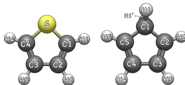
Fig. 3 Structure and labeling of thiophene and cyclopentadiene.
