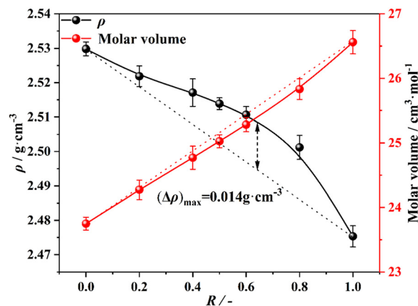
Fig. 5 Compositional dependence of the density ( \rho ) and molar volume of the 65.0\text{SiO}_2 \cdot 5.0\text{B}_2\text{O}_3 (17.6 - x) \cdot \text{Na}_2\text{O} \cdot x\text{K}_2\text{O} \cdot 7.5\text{CaO} \cdot 4.9\text{MgO} glasses as a function of different molar ratios R , where R is equal to the molar ratio of [\text{K}_2\text{O}]/([\text{Na}_2\text{O}] + [\text{K}_2\text{O}]) . The dashed line is a guide for the eye.
