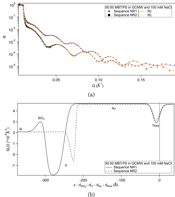
Fig. 2 (a) NR curves for the two samples of 50 : 50 MBT : PS, with best fit lines. Error bars are shown on the data points. Differences in reflectivity are mainly due to the different characteristics of the gold-coated substrates. (b) Corresponding SLD profiles. The layers considered in the slab model are indicated. In the case of the substrate used in sequence NR2, there was some mixing of the Ti and SiO 2 layers, as shown by the less defined peaks in the profile. The zero on the x-axis is placed at the thiol/solution interface, so that the portions of the profiles relative to the thiol layer are aligned despite differences in the substrates.
