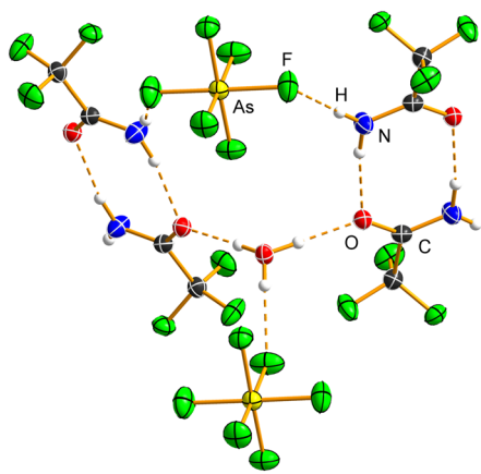
Fig. 5 R 6 4 (14) hydrogen-bonded cluster in the crystal structure of the H 3 O[AsF 6 ] 2 CF 3 CONH 2 salt cocrystal. Hydrogen bonds are shown by dashed orange lines. Displacement ellipsoids are drawn at the 50% probability level, and hydrogen atoms are represented as spheres of arbitrary radius.
